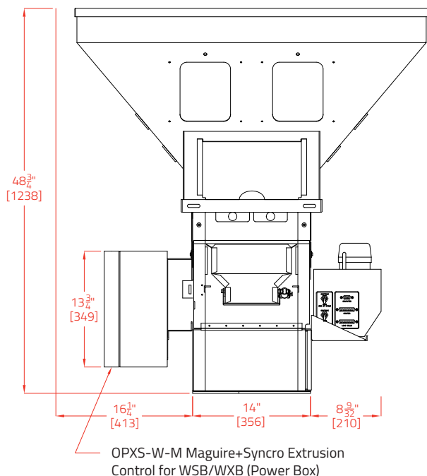
WXB-240 FRONT VIEW
