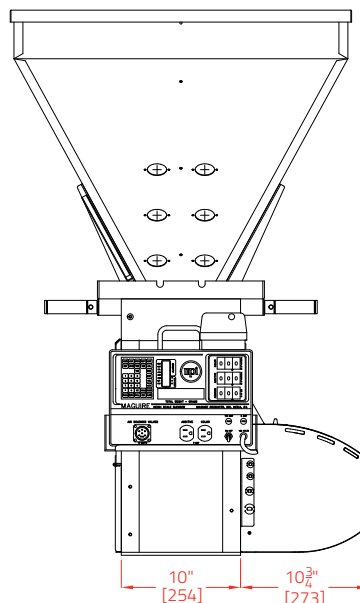
WXB-240 SIDE VIEW
